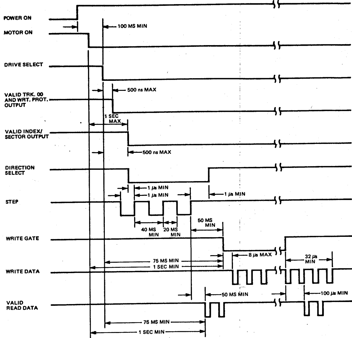
FIGURE 8. GENERAL CONTROL AND DATA TIMING REQUIREMENTS
