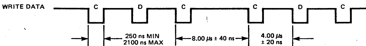
FIGURE 7. WRITE DATA TIMING
