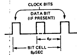
FIGURE 18. BIT CELL
