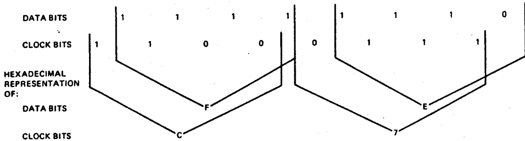
FIGURE 22. ID ADDRESS MARK
