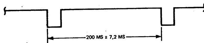
FIGURE 11. INDEX SECTOR TIMING (SA104 MEDIA)
