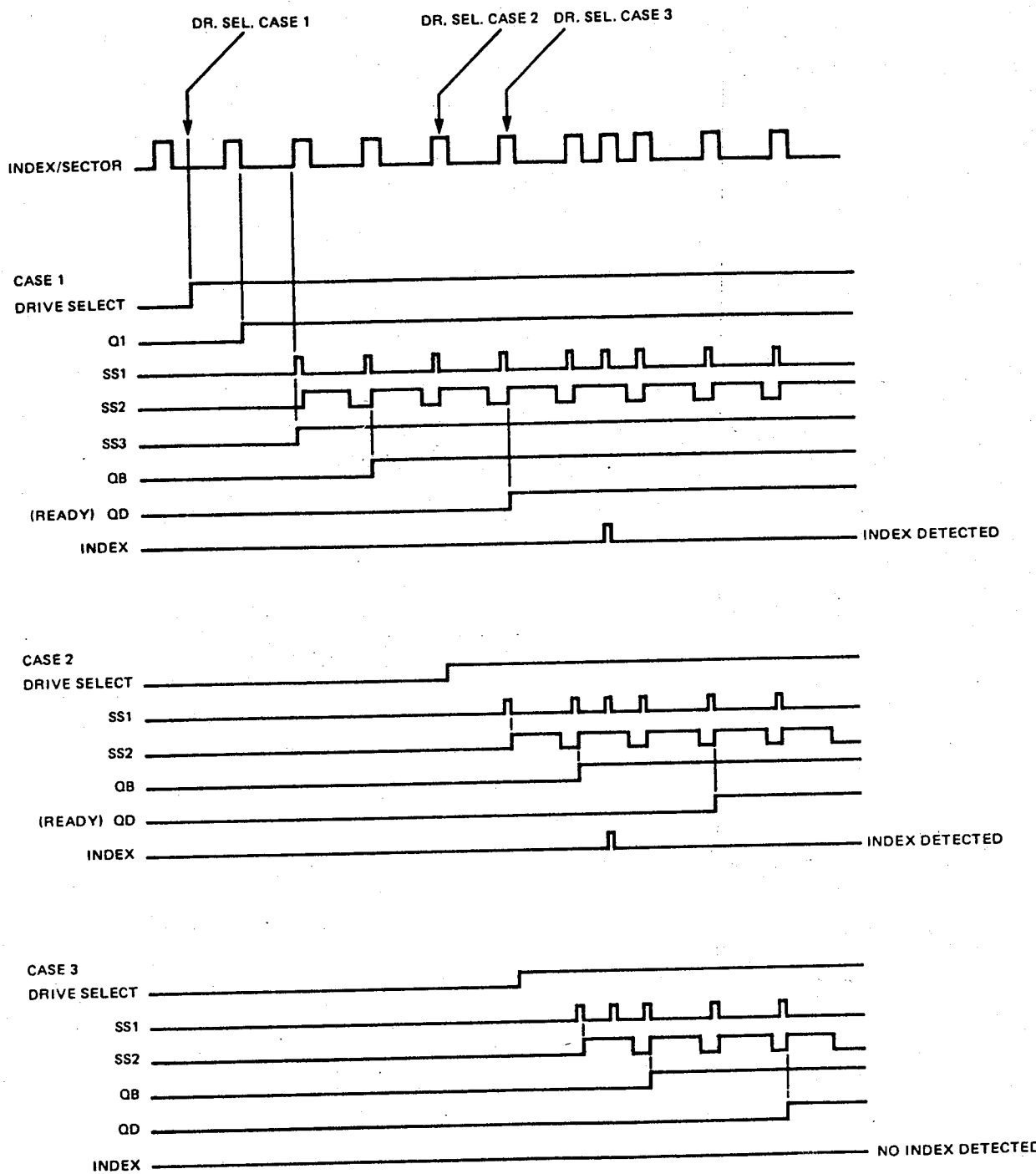
FIGURE 35. INDEX/SECTOR TIMING
