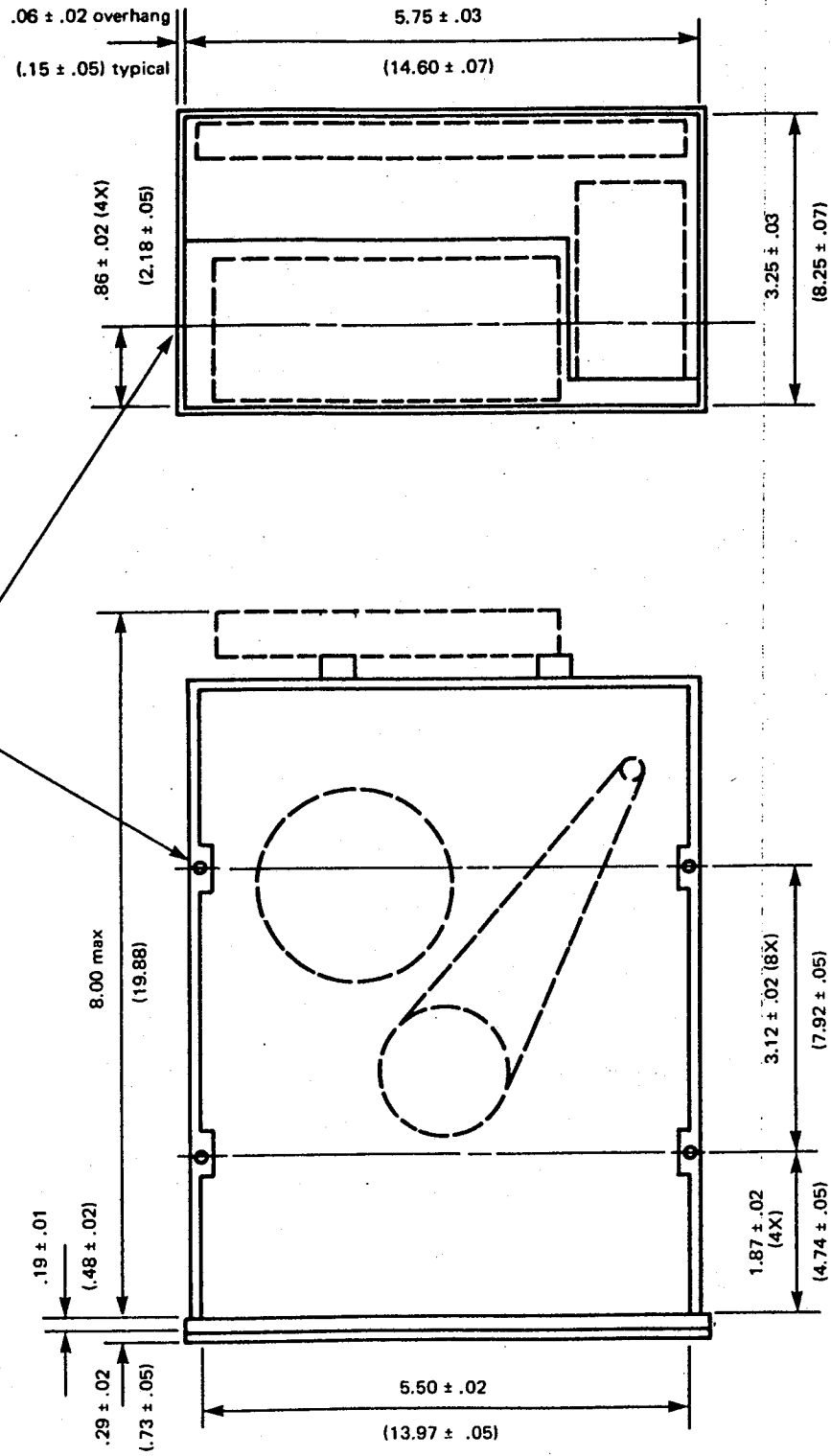
FIGURE 16. SA400 DRIVE DIMENSIONS
