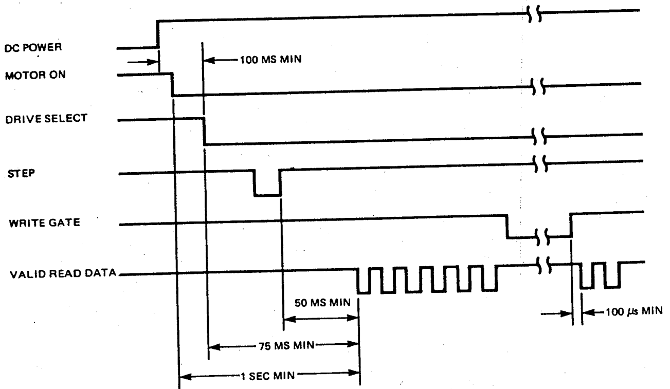
FIGURE 4. READ INITIATE TIMING
