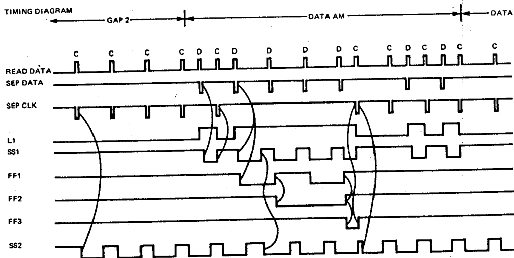
FIGURE 29. TRUE DATA SEPARATOR
