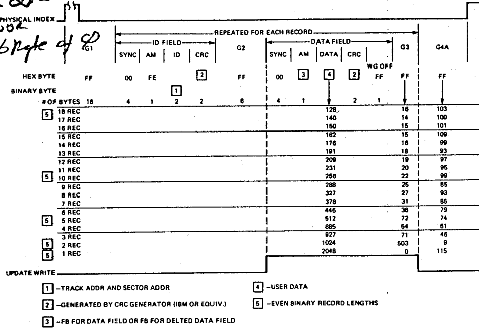
FIGURE 25. SOFT SECTORED FORMATS
