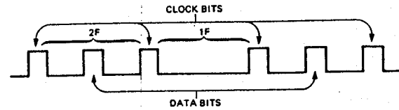
FIGURE 17. DATA PATTERN
