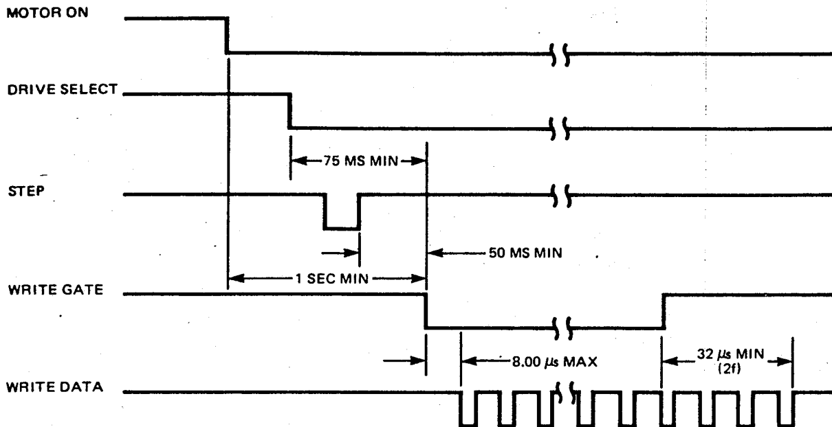
FIGURE 6. WRITE INITIATE TIMING
