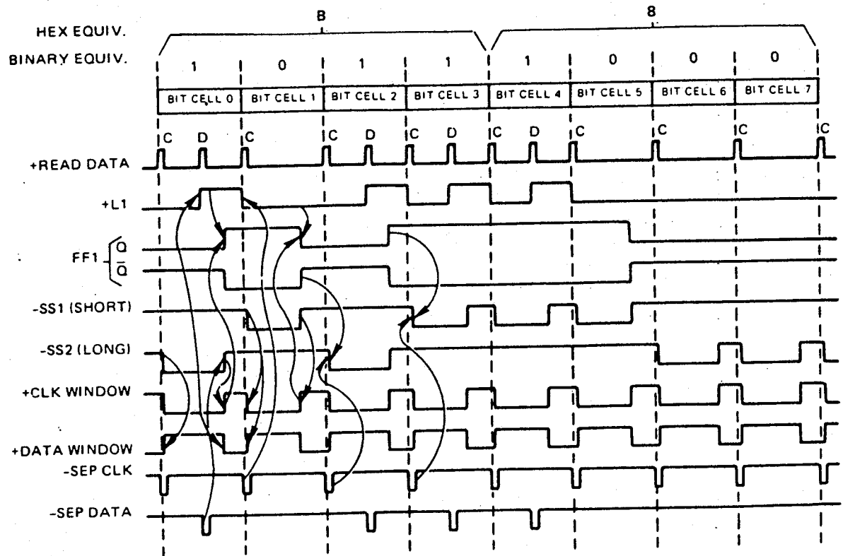
FIGURE 28. DATA SEPARATOR TIMING DIAGRAM
