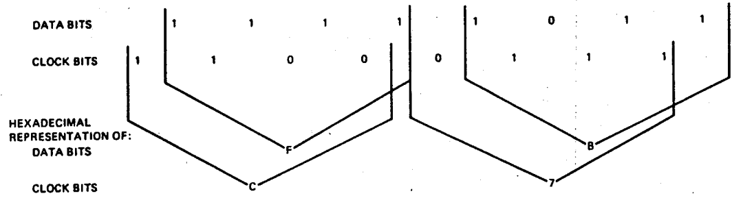
FIGURE 23. DATA ADDRESS MARK
