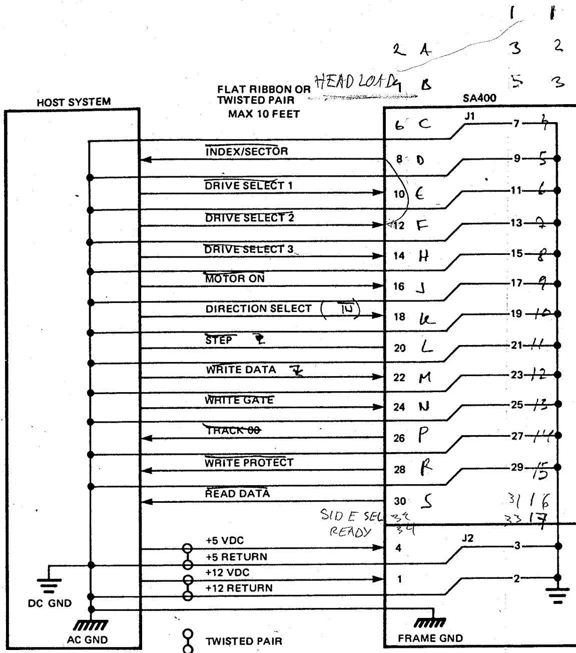
FIGURE 9. INTERFACE CONNECTIONS
