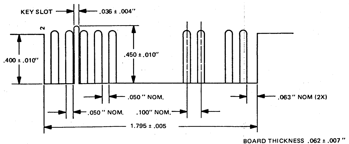
FIGURE 13. J1 CONNECTOR DIMENSIONS
