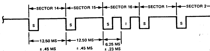
FIGURE 12. INDEX SECTOR TIMING (SA105 MEDIA)
