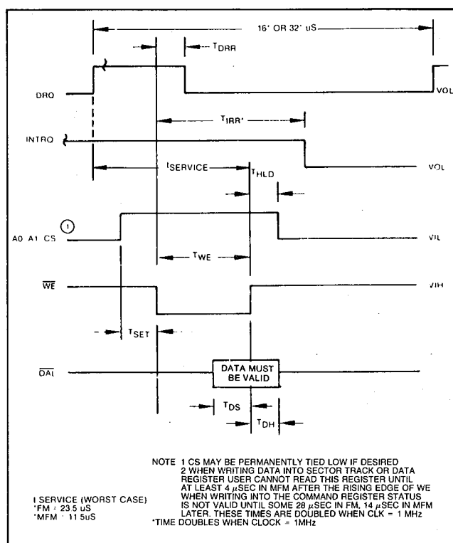
WRITE ENABLE TIMING
