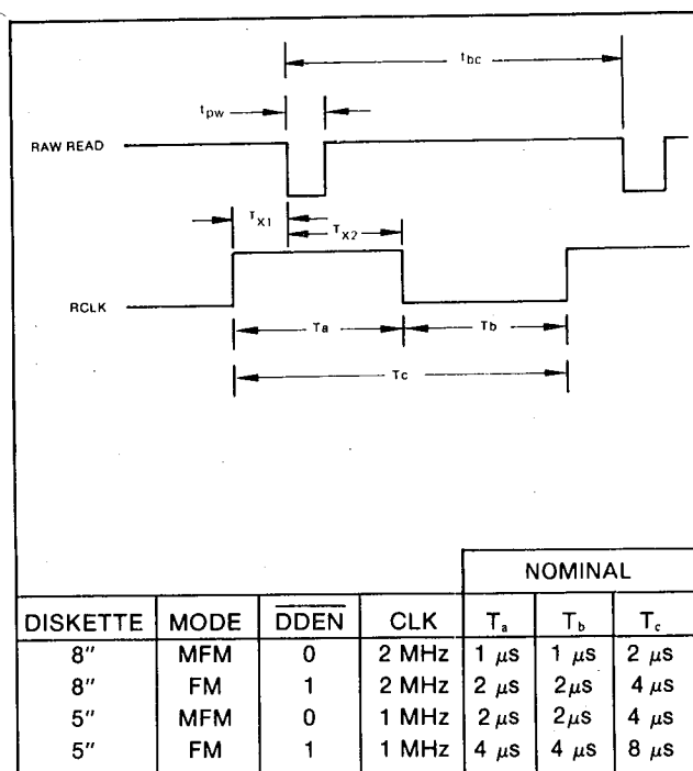
INPUT DATA TIMING
