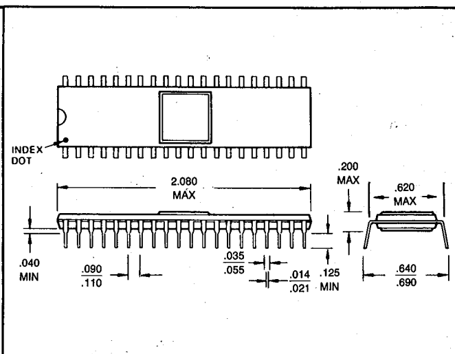
FD179XB-02 PLASTIC PACKAGE
